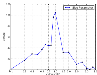
Figure 6: Sensitivity of parameter c .
